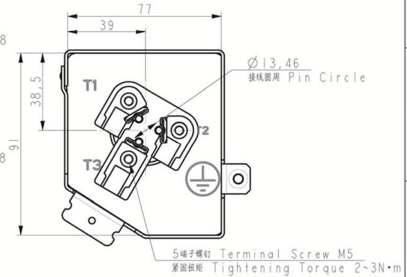
接线盒布置 T-Box Layout Standard
