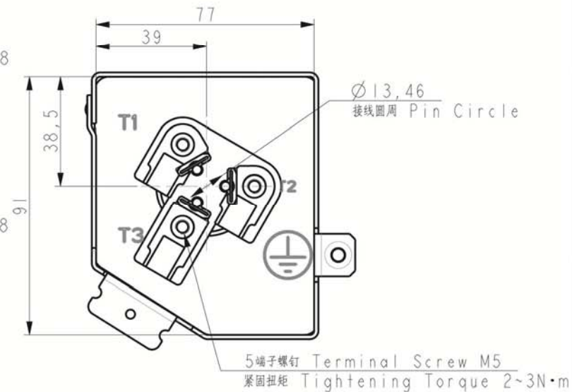
接线盒布置 T-Box Layout Standard
